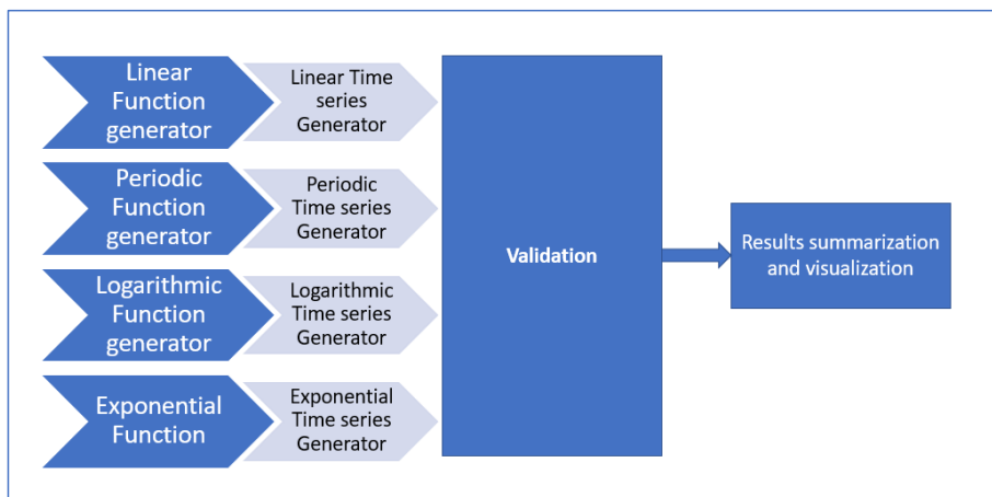
Figure 3: Data generation and evaluation pipeline
