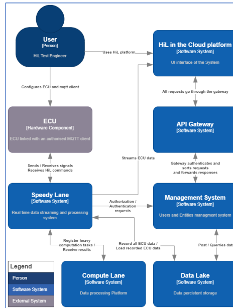
Figure 1: High level diagram of HiL in the cloud.
