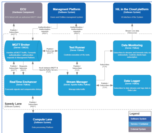
Figure 2: Deployment diagram of Speedy Lane of HiL in the cloud platform
